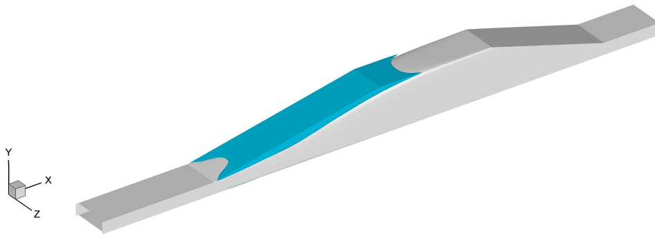
Figure 4.5 Case 2: Isosurface of Separation with \overline{v^2} - f Model
