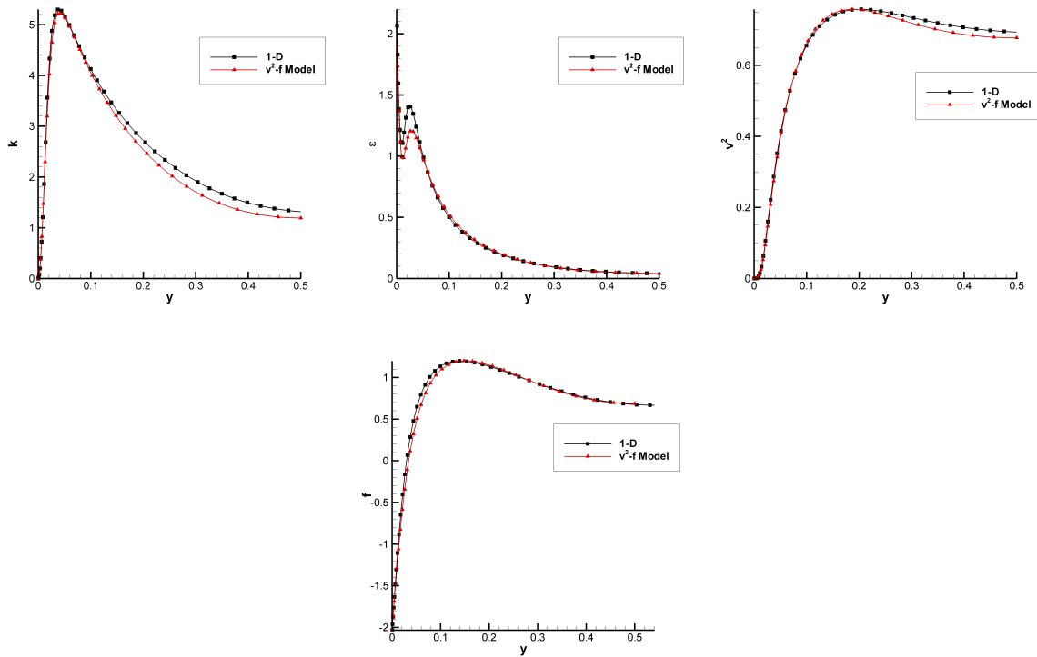
Figure 3.5 Case 1: Turbulence Quantities with \overline{v^2} - f Model
