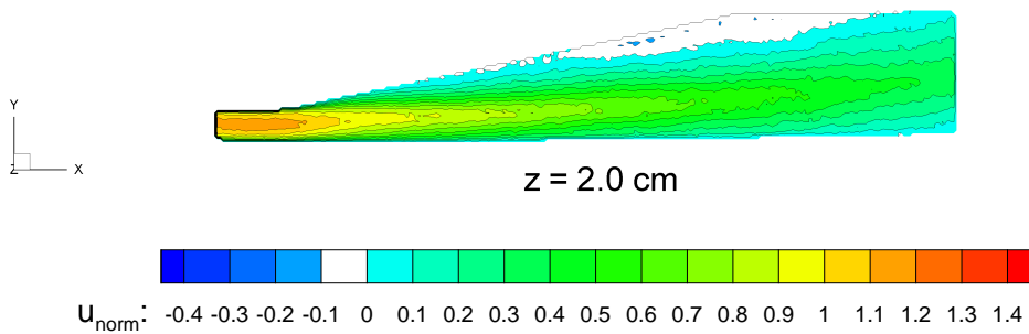
Figure 5.6 Case 3: Experimental Contours of Streamwise Velocity at z = 2 cm
