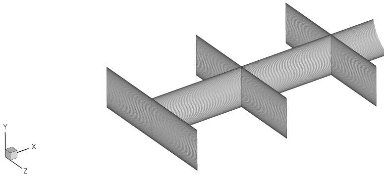
Figure 3.1 Case 1: Numerical Grid 3-D View
