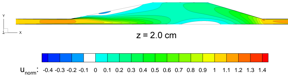
Figure 5.15 Case 3: Contours of Streamwise Velocity at z = 2 cm with v^2 - f Model
