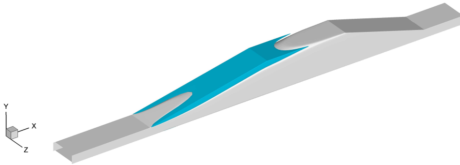
Figure 4.6 Case 2: Isosurface of Separation with \zeta - f Model
